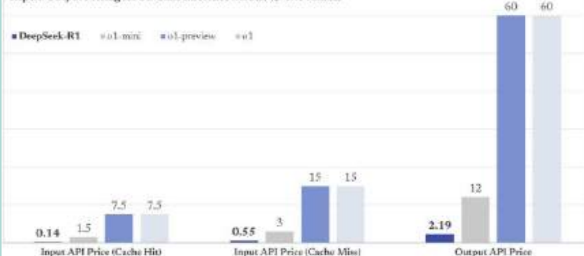
Input/Output Pricing for o1-Class Inference Models ($/1M Tokens)
